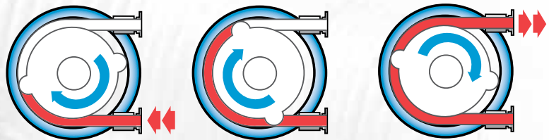
Peristaltic Pump Principle
