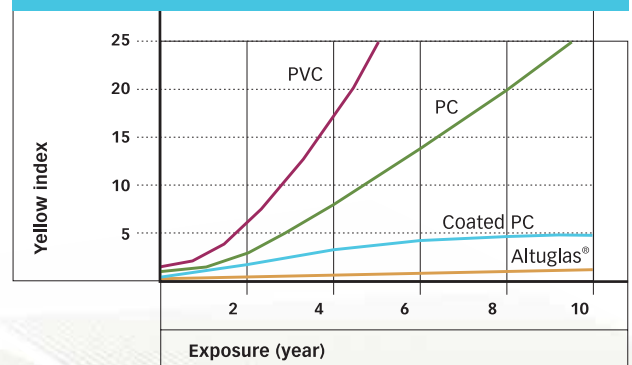
Variation in the yellow index as a function of exposure to weathering.
