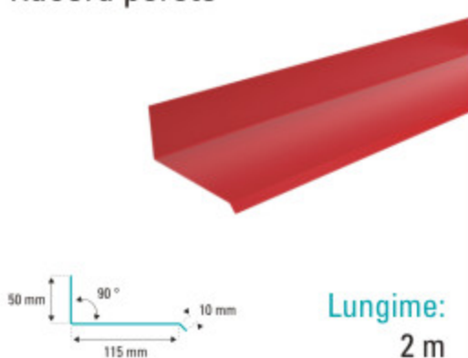
Racord perete
