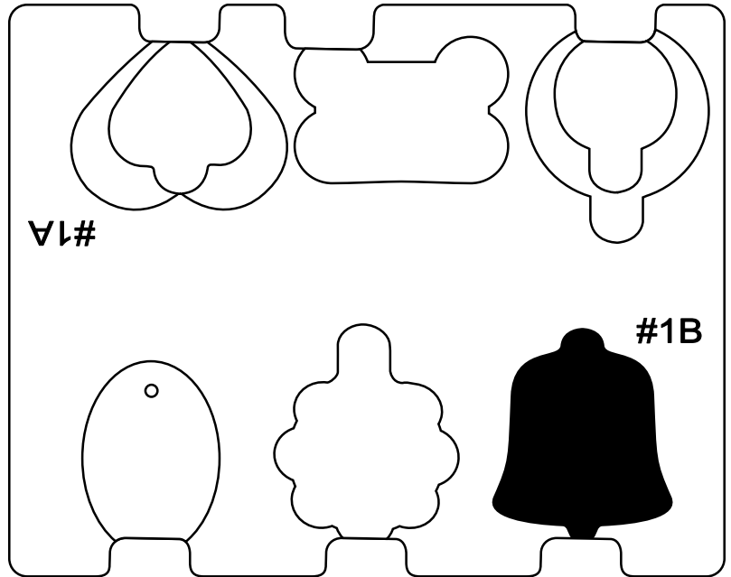
Fixture p/n 11238-01
