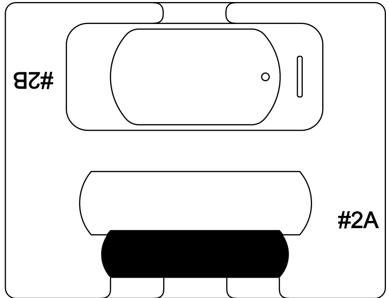
Fixture p/n 11238-02
