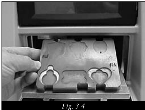
Fig. 3-4 Install the tag holder onto the platform with the style to be engraved to the front.
