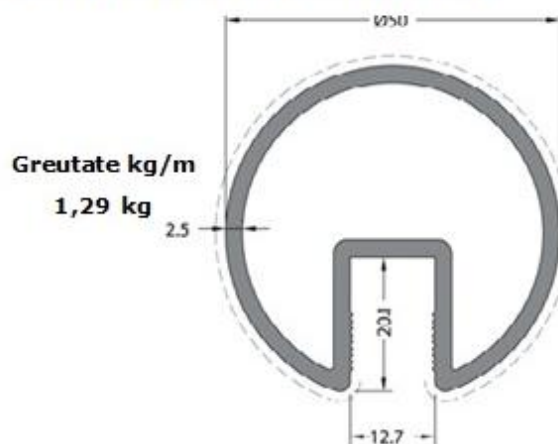
Mana curenta balustrada sticla
