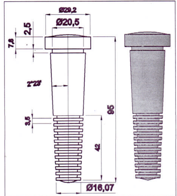
DEGET DEPLUMATOR - MODEL 2; L=95 mm
