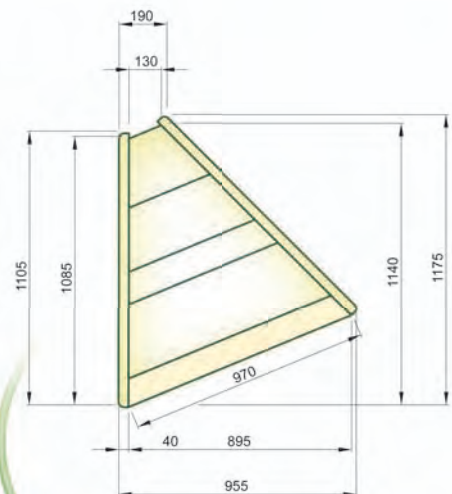
LDG-NZ45-05
