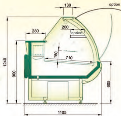
LSG-xxx-05
