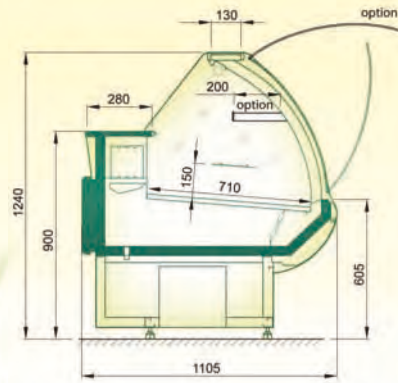
LDG-xxx-05
