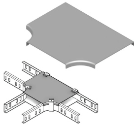
mountaing scheme
