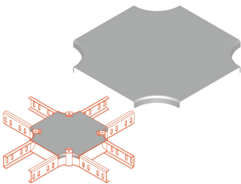
mountaing scheme
