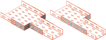
mountaing scheme
