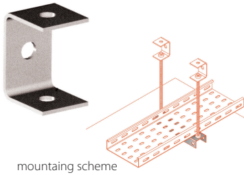
mountaing scheme
