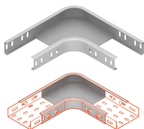
mountaing scheme
