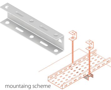
mountaing scheme
