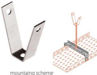
mountaing scheme
