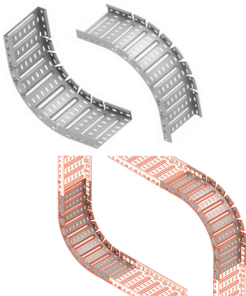
mountaing scheme
