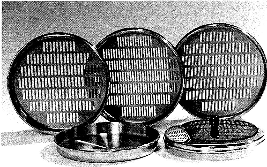
Analytical sieves according to ISO 5223
