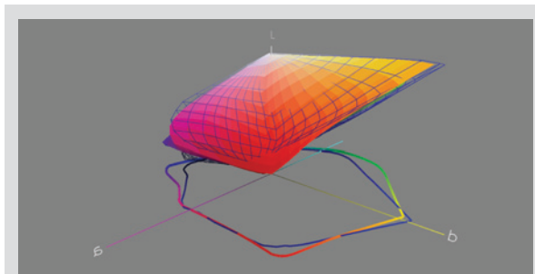
The color gamut chart above shows in detail the wider gamut of reds that the HP Designjet Z3200 Photo Printer (in solid) achieves in comparison to one of its competitors. HP Premium Instant-dry Gloss Photo Paper was used for the demonstration.
