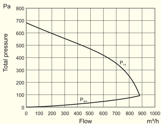
GSF-2-160/62-018S AP HT
