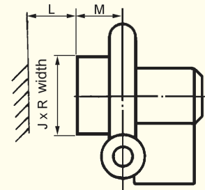
Filter silencer Type B
