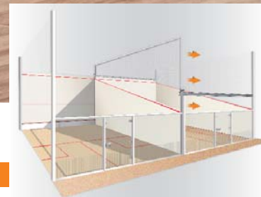
CT FLEXI Court in der Single-Position
