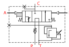
BZDP 180C (Tirador/Puller) 9036090/2
