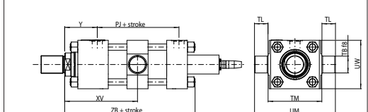
L (ISO MT4) = intermediate trunnion
