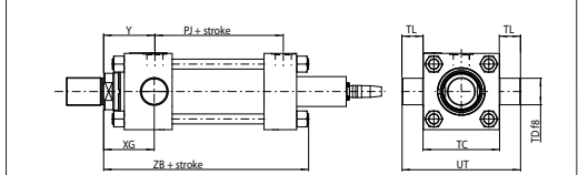
G (ISO MT1) = front trunnion
