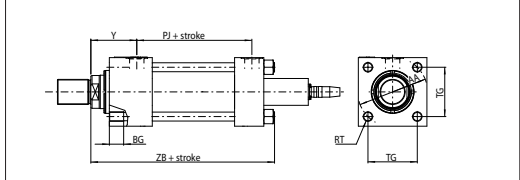
Z (ISO MX5) = front threaded holes
