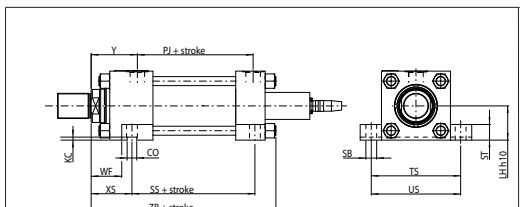
E (ISO MS2) = feet
