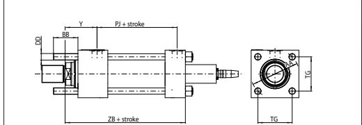
Y (ISO MX3) = front tie rods extended
