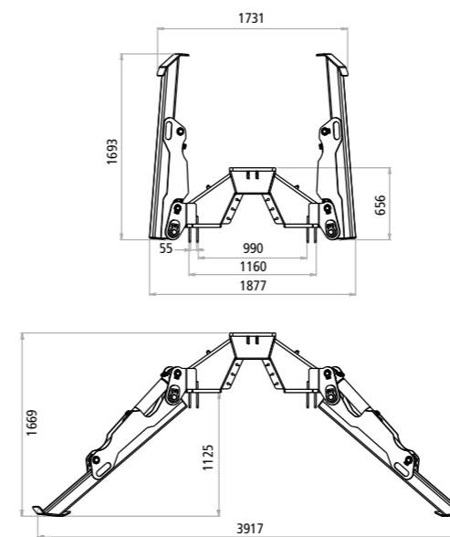
Flap-down stabiliser legs
