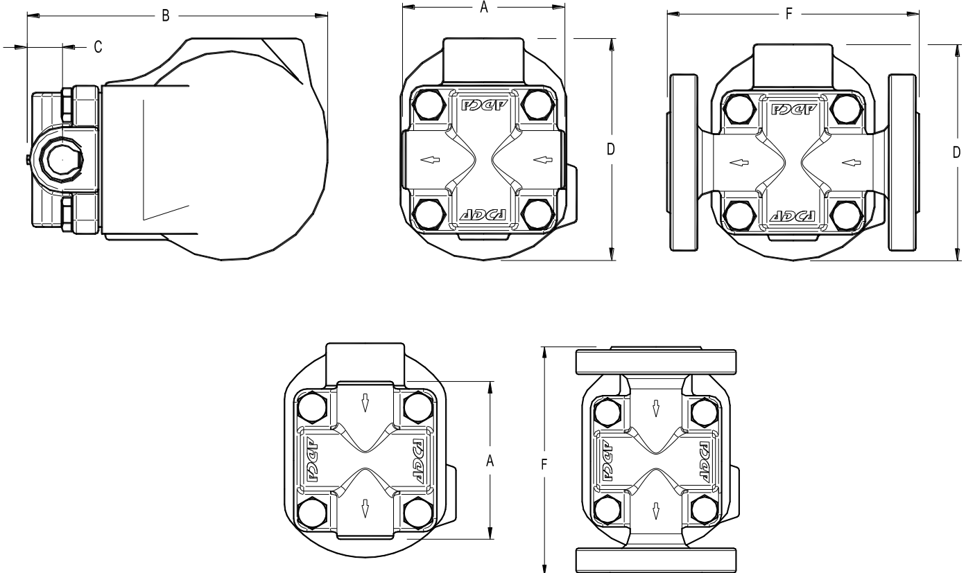
Vertical Installation (V)
